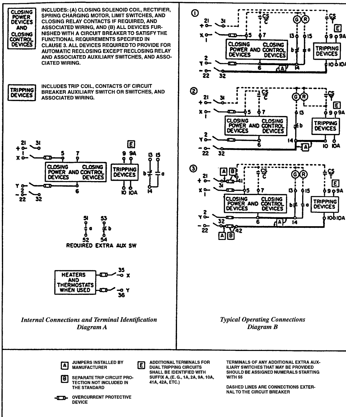
Figure 2—Circuit breaker intended for use in metal-clad switchgear, where
