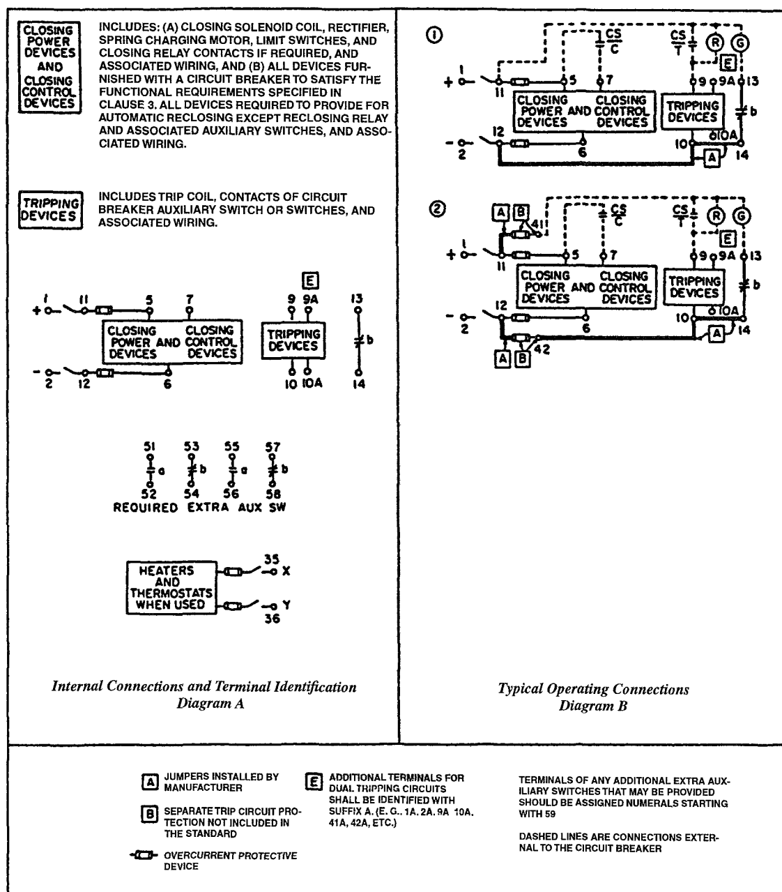
Figure 1—Circuit breaker intended for use in metal-clad switchgear, where
