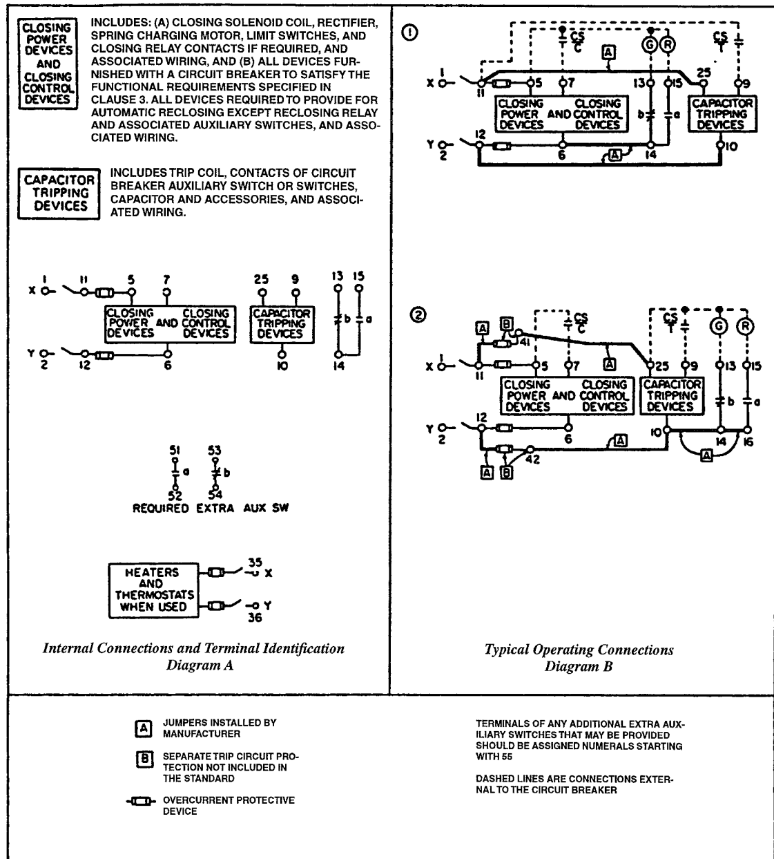
Figure 3—Circuit breaker intended for use in metal-clad switchgear, where —The closing power is ac —The closing control is ac —The tripping control is by capacitor tripping devices
